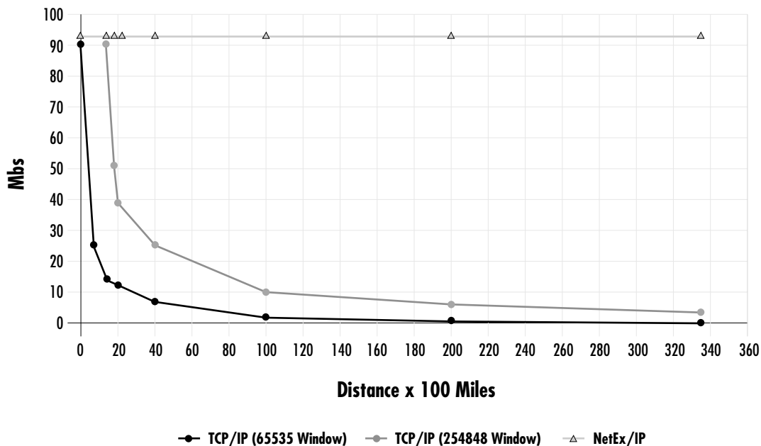
NetEx/IP vs TCP/IP Performance over Fast Ethernet Interface (100 Mb/s) Max Capacity
